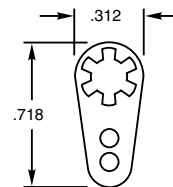
Pierced Terminal
