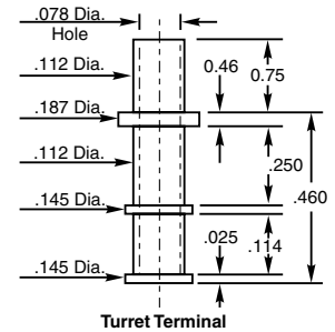
Turret Terminal
