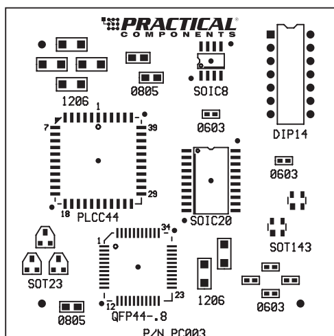
PCB003 Solder Practice Board
