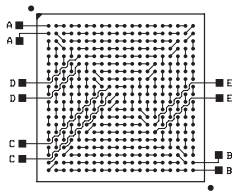
PBGA 256/272/300/316/356-27MM
