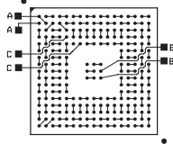
PBGA 208/217/240/249-23MM
