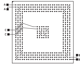
PBGA 352/388-35MM
