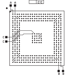
PBGA 304/329-31MM
