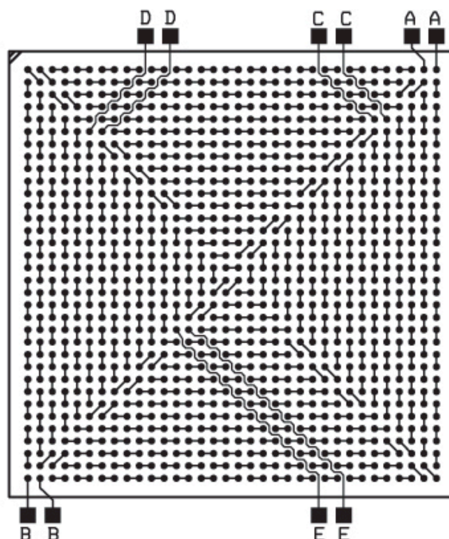
PBGA 580/680/1156-35MM
