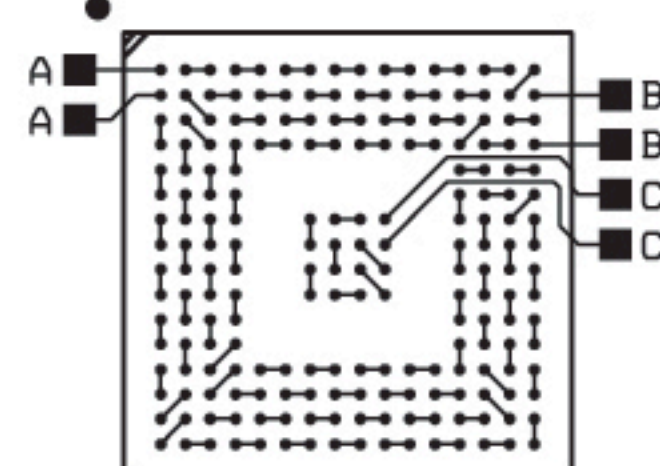
PBGA 156/160-15MM PBGA 192/208-17MM
