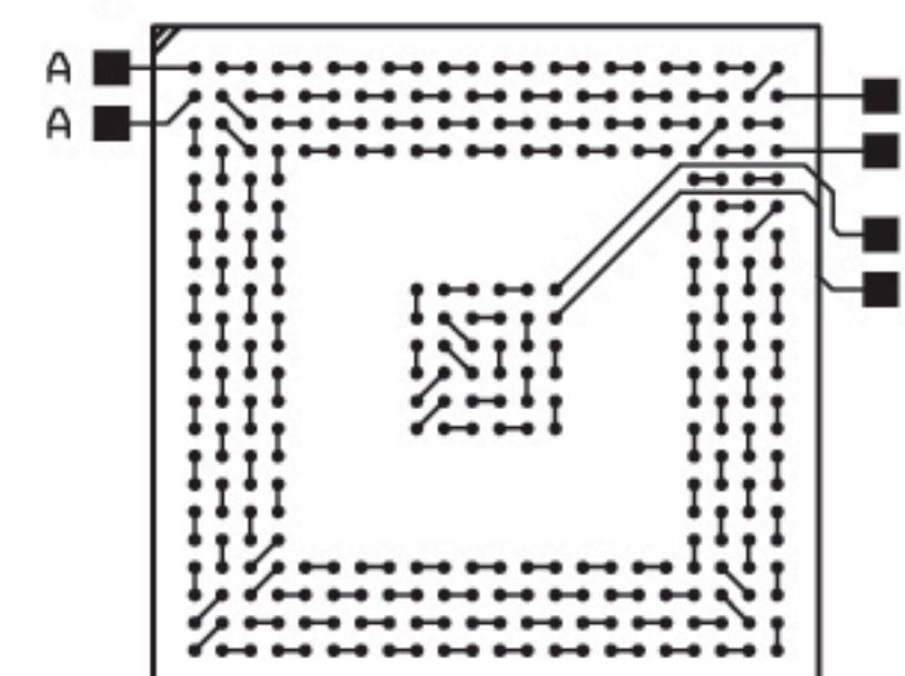
PBGA 288/324-23MM
