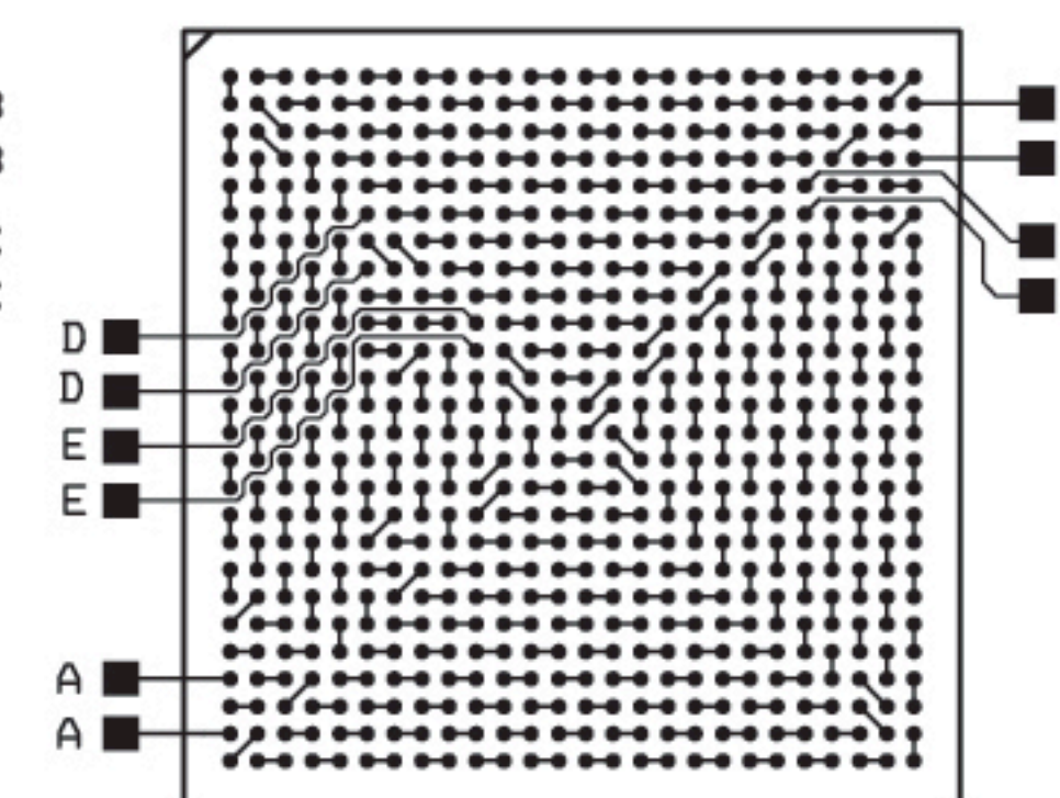
PBGA 416/484/676-27MM
