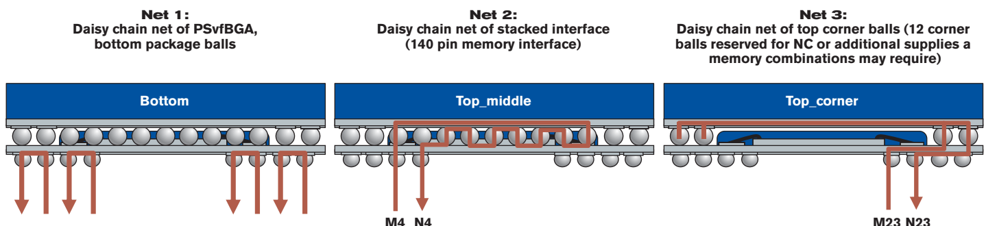
4 . This figure illustrates the three-net design used in our PoP daisy chain components to enable electrical monitoring of the bottom and top BGA locations critical in PoP stacking and board-level reliability testing.
