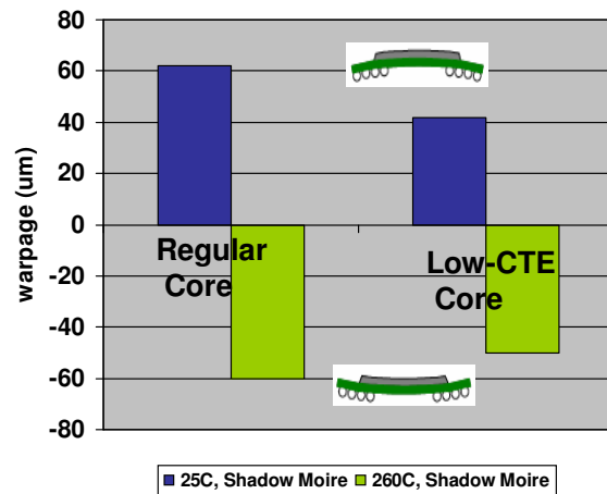
Figure 5 Low-CTE core substrate warpage
