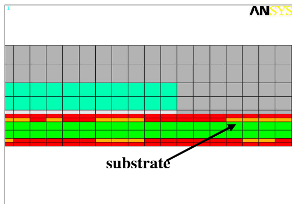
Figure 15 Detailed Substrate Layer Model
