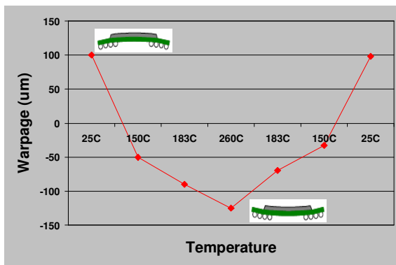
Figure 3 14mm PSvfBGA warpage profile
