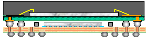
Figure 8 PSfcCSP PoP
