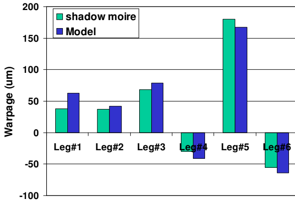
Figure 17 Simulation vs. shadow moiré warpage at 25C
