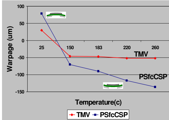
Figure 10 Warpage of TMV vs PSfcCSP
