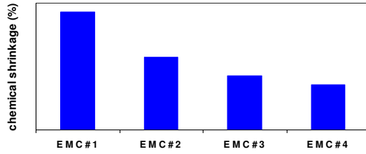
Figure 14 EMC chemical shrinkage data
