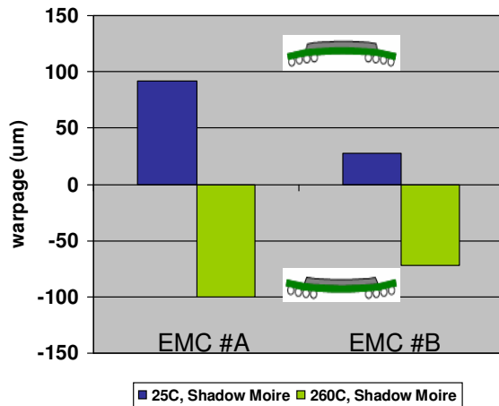
Figure 6 Effect of EMC material property
