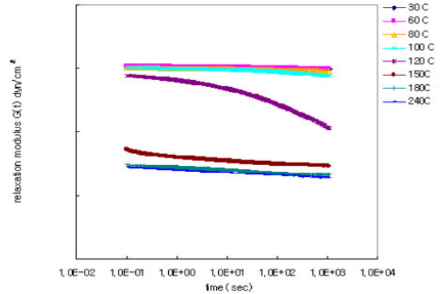
Figure 12 Stress relaxation curves at 8 different temperatures
