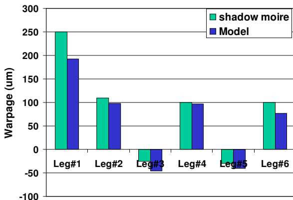
Figure 18 Simulation vs. shadow moiré warpage at 260C
