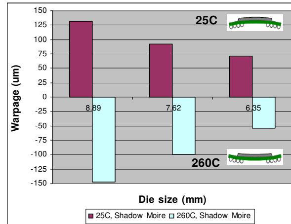
Figure 7 Effect of die size on 14mm package warpage
