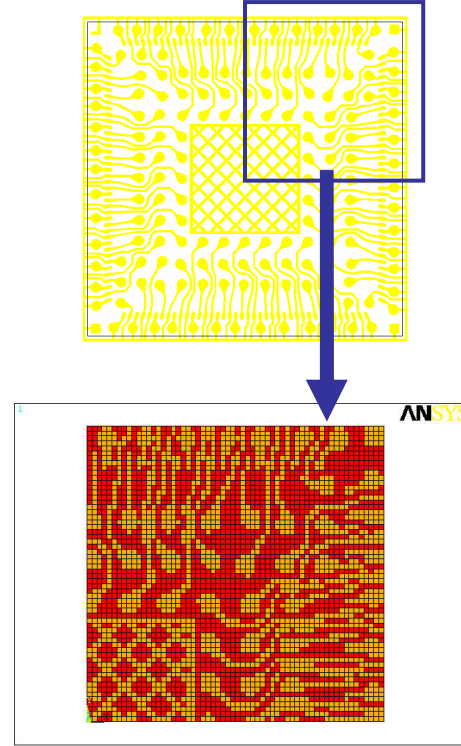
Figure 16 Example of Signal Layer Layout Model
