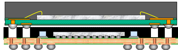
Figure 9 Thru-Mold-Via (TMV) technology
