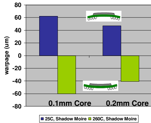
Figure 4 Warpage of 0.1mm core vs 0.2mm core
