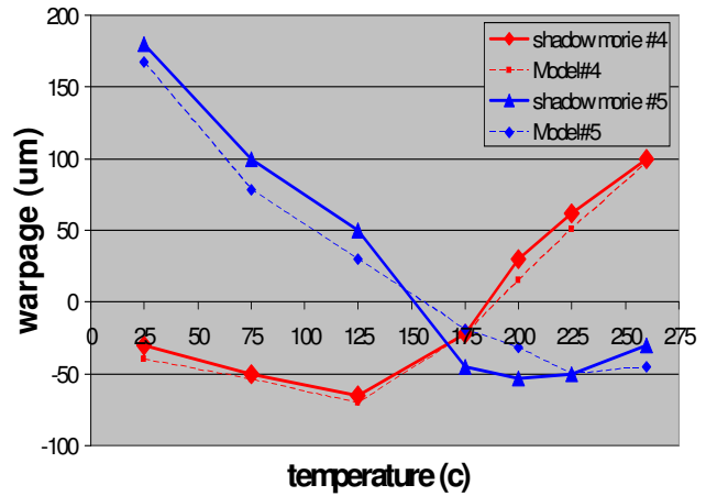
Figure 19 Simulation vs. shadow moiré over the entire temperature range
