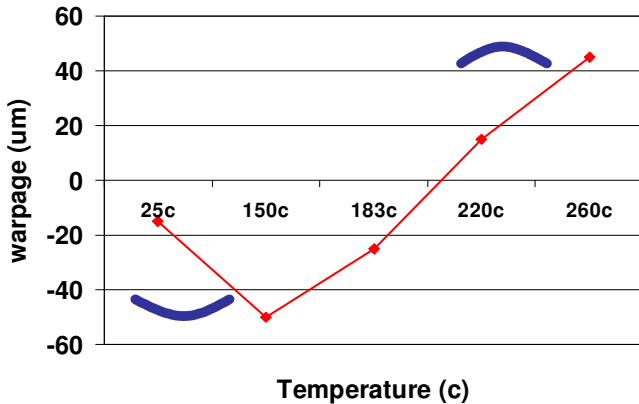
Figure 11 Top SCSP warpage from 25C to 260C
