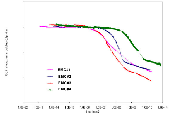
Figure 13 Master curves of 4 EMCs measured
