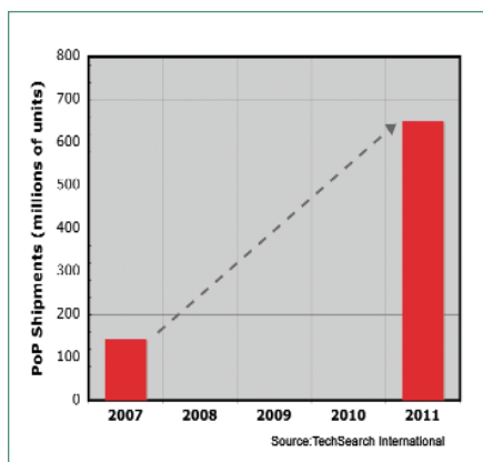
Figure 1. TechSearch International is forecasting a 40 percent CAGR for PoP through 2012.
