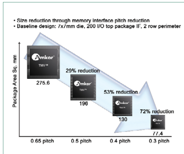
Figure 7. Size reduction benefits of PoP
