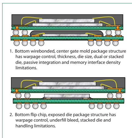
Figure 4. This graphic illustrates limitations of current bottom PoP technologies.
