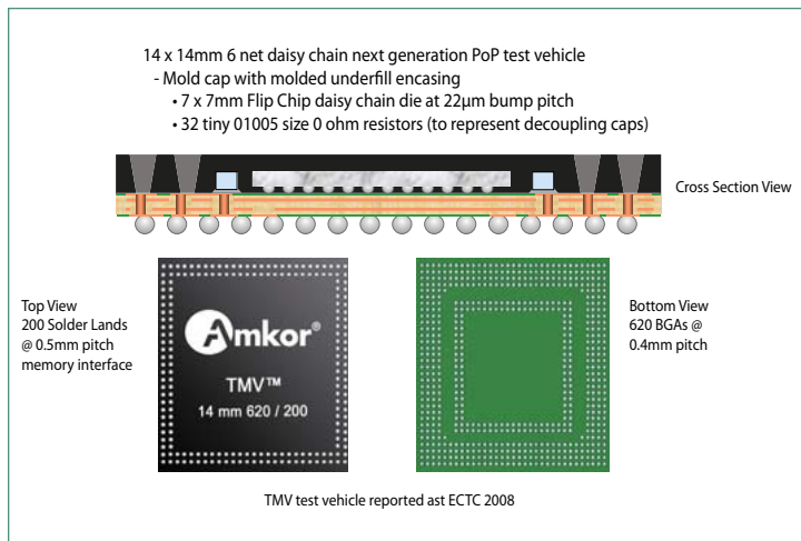
Figure 6. This is the high density, six-net daisy chain test vehicle reported at ECTC.
