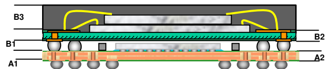
Figure 7. PSfcCSP Test Vehicle
