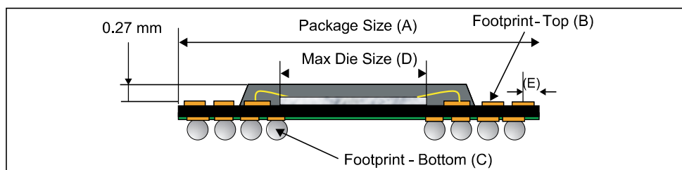
PSvfBGA Design Table for 0.65 mm Pitch 2 Row Stacked Interfaces
