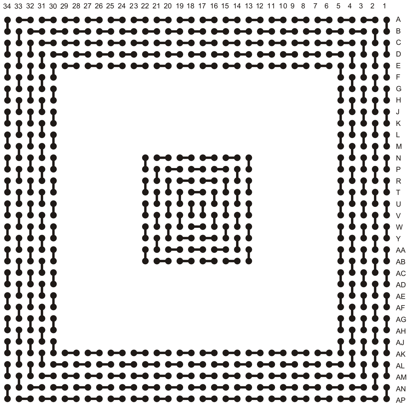
A-PBGA680-1.0mm-35mm
