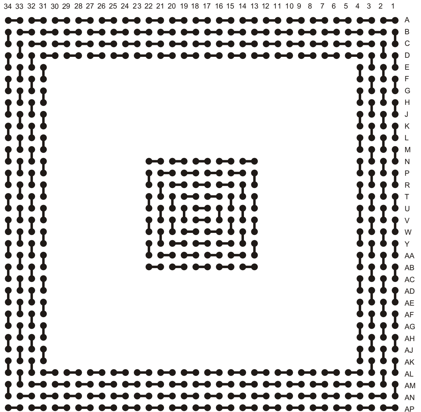
A-PBGA580-1.0mm-35mm-DC
