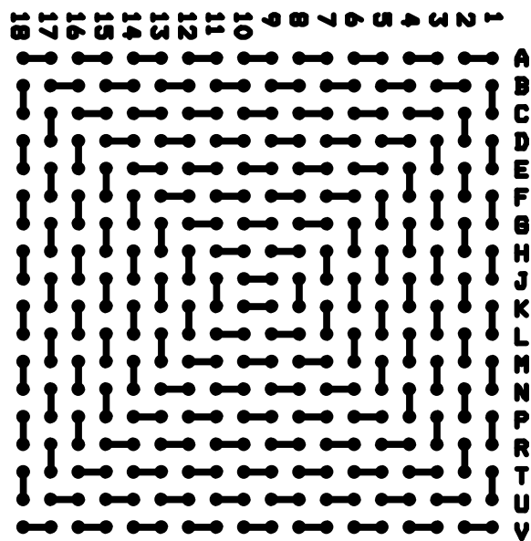
BOTTOM VIEW PBGA324-1.0-19MM
