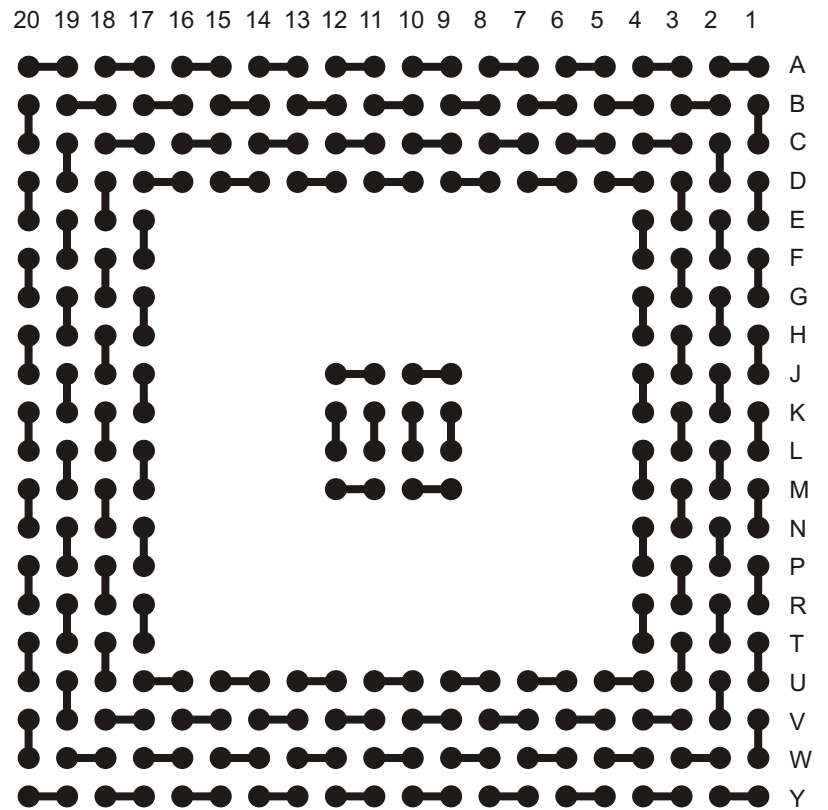
A-PBGA272-1.27mm-27mm Ball View
