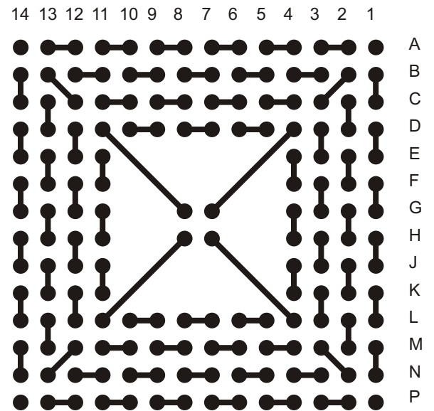
A-PBGA160-1.0mm-15mm-DC
