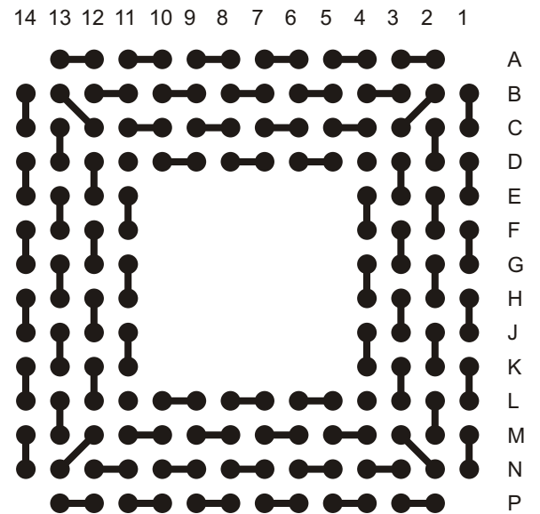
A-PBGA156-1.0mm-15mm-DC SID# 101303620 Ball View
