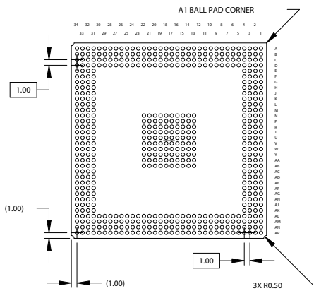
BOTTOM VIEW 580 SOLDER BALLS
