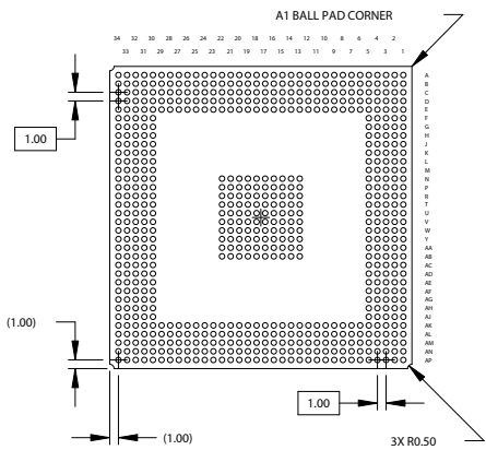
BOTTOM VIEW 680 SOLDER BALLS
