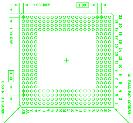
BOTTOM VIEW (286 SOLDER BALLS)
