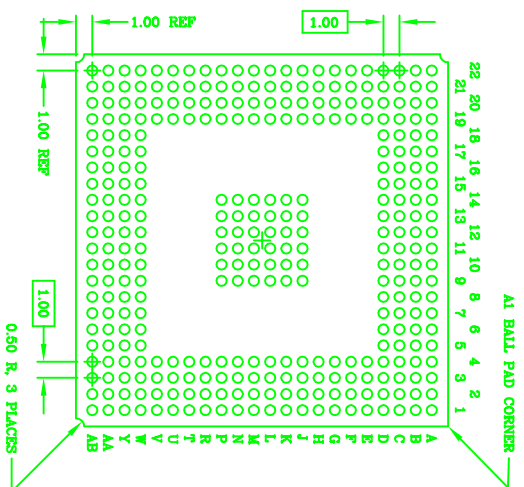
BOTTOM VIEW (324 SOLDER BALLS)
