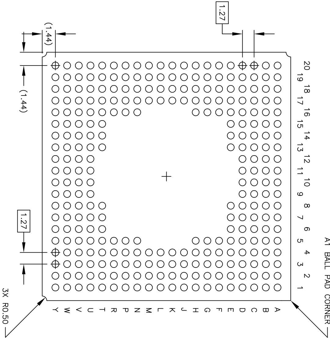
BOTTOM VIEW 284 SOLDER BALLS
