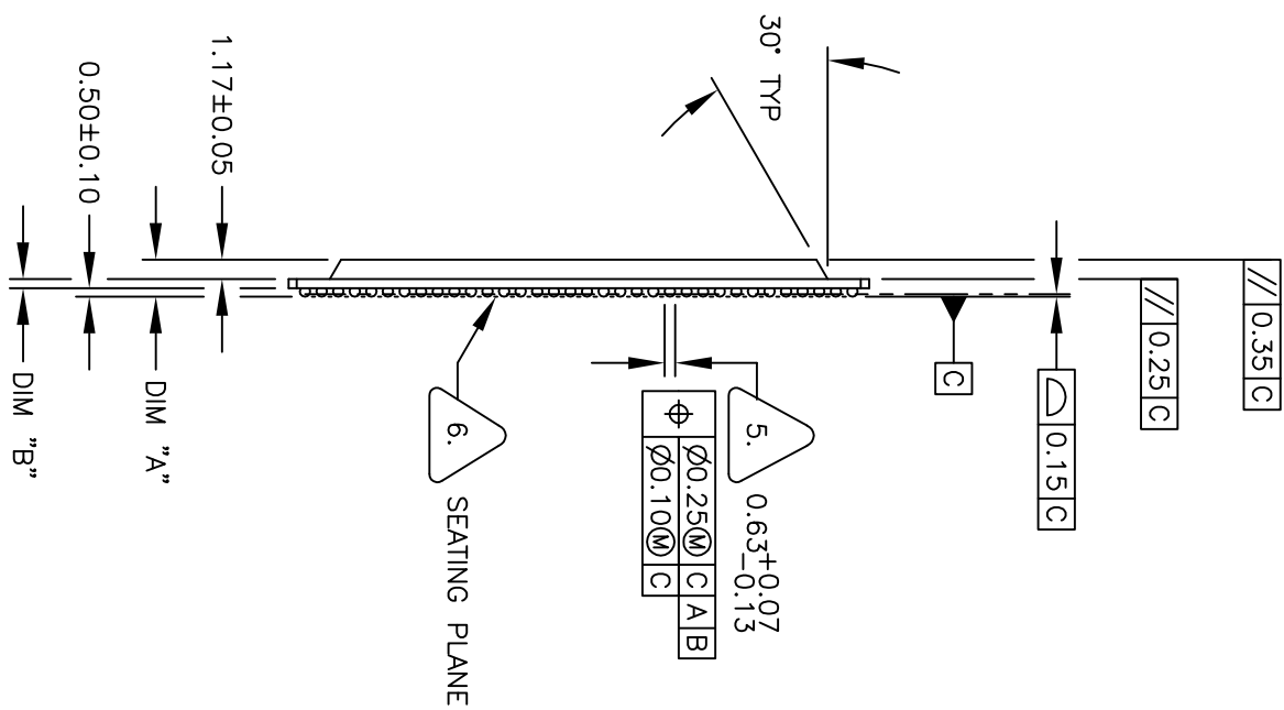
SIDE VIEW
