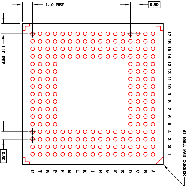
BOTTOM VIEW (206 SOLDER BALLS)
