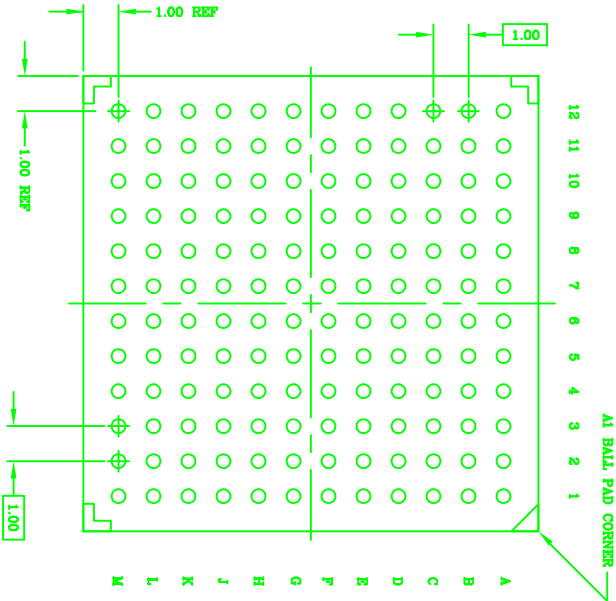
BOTTOM VIEW (144 SOLDER BALLS)
