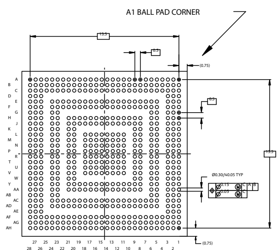
DIE BOTTOM / BALL SIDE VIEW 604 SOLDER BALLS
