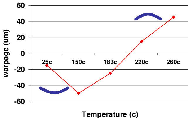
Figure 11 Top SCSP warpage from 25C to 260C
