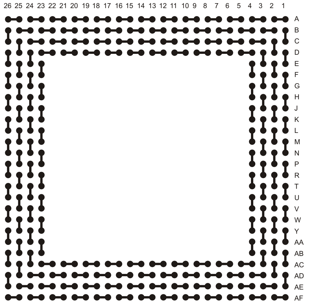
PBGA352-1.27mm-35mm-DC-ASE
