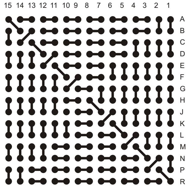
PBGA225-1.5mm-27mm-DC
