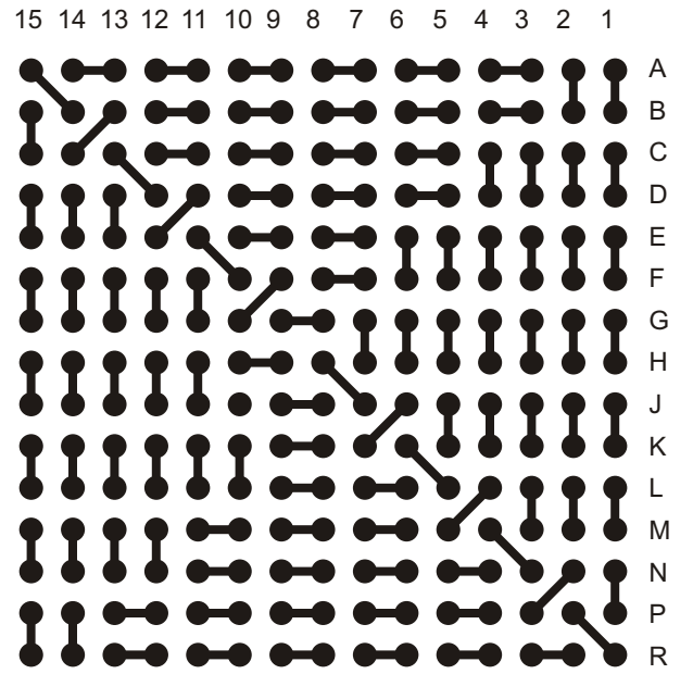
PBGA225-1.5mm-27mm-DC
