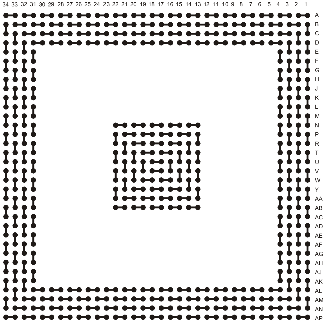
A-PBGA580-1.0mm-35mm-DC
