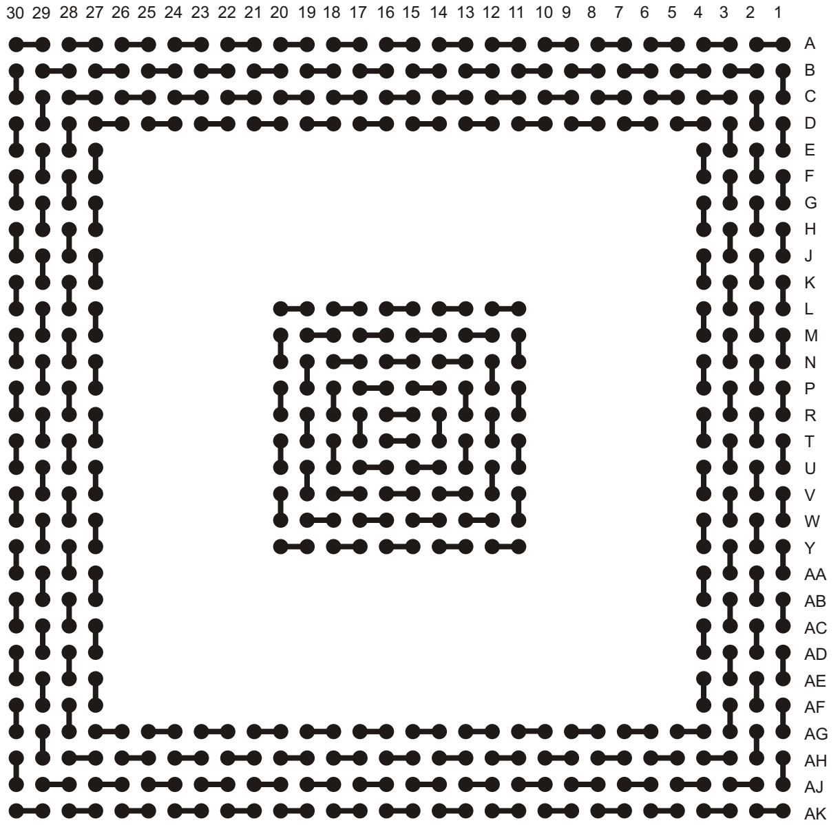
A-PBGA516-1.0mm-31mm Ball View
