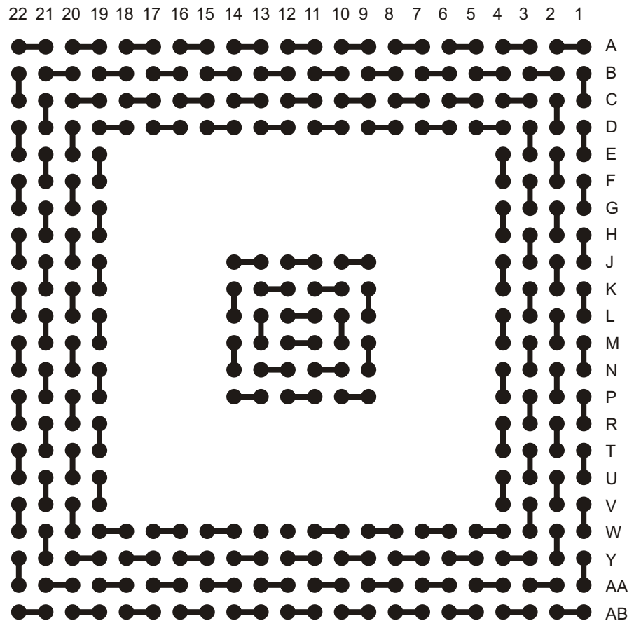
A-PBGA324-1.0mm-23mm-DC SID #101301999 Ball View
