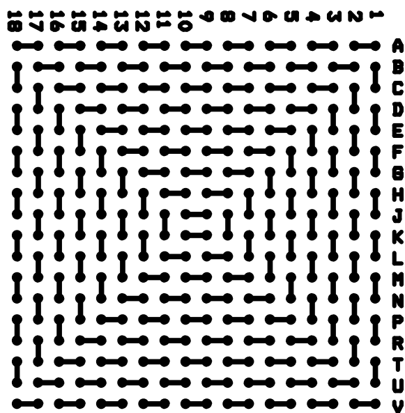
BOTTOM VIEW PBGA324-1.0-19MM
