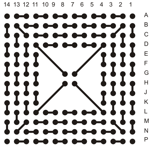
A-PBGA160-1.0mm-15mm-DC Ball View
