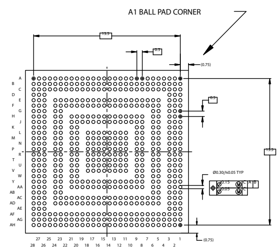
DIE BOTTOM / BALL SIDE VIEW 604 SOLDER BALLS
