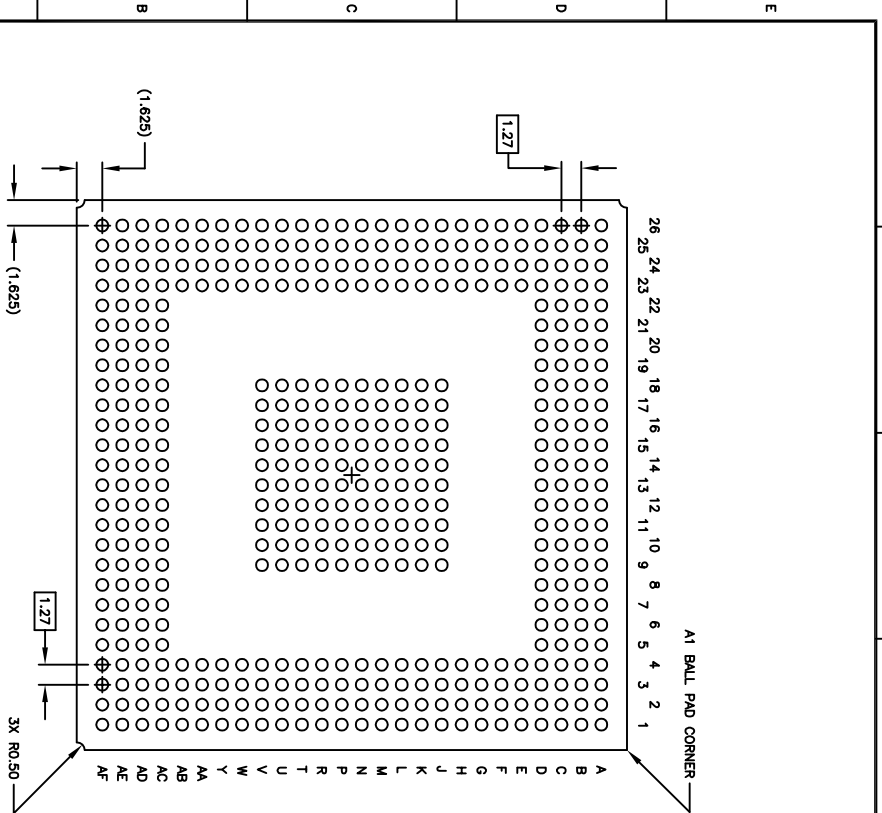
BOTTOM VIEW 452 SOLDER BALLS
