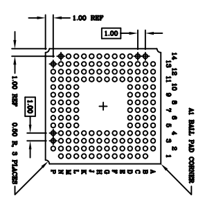
BOTTOM VIEW 156 SOLDER BALLS
