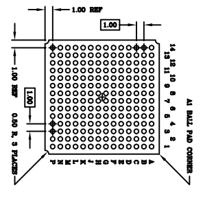
BOTTOM VIEW 196 SOLDER BALLS
