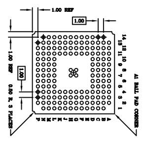
BOTTOM VIEW 160 SOLDER BALLS
