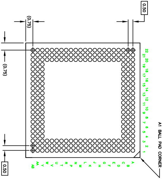
BOTTOM VIEW (228 SOLDER BALLS)
