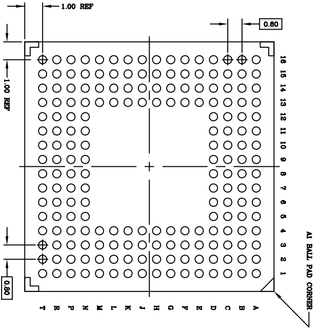
BOTTOM VIEW (192 SOLDER BALLS)
