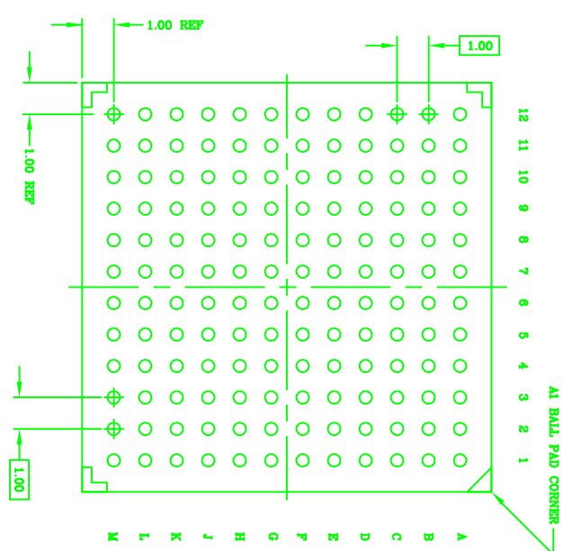
BOTTOM VIEW (144 SOLDER BALLS)
